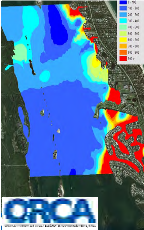
Total nitrogen map of the study area. This gradient map shows the total nitrogen (mg/kg) of sediment samples collected in Indian River County.
